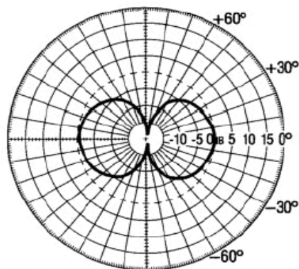
Diagrama de Radiación Vertical Vertical Radiation Pattern
